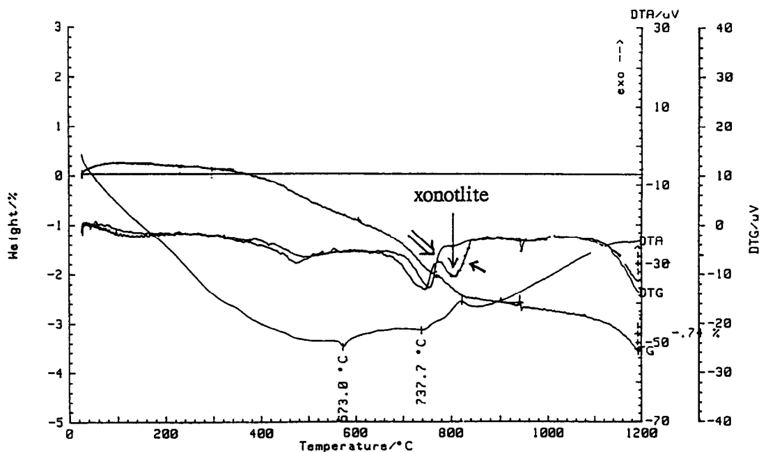
FIG 5 : Thermogravimetric curve of BQ400°C/P → DTG of sample taken from the inner part of test piece ⇒ DTG of sample taken in periphery of test piece
